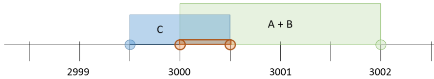
Figure 2. Overlap of intervals
